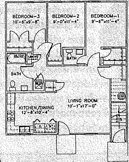
(1st Floor Plan) THREE BEDROOM 1 1/2 BATH APARTMENT PLAN 1004 SQ. FEET
