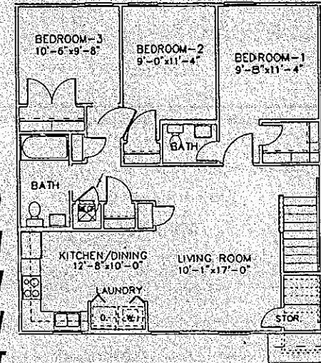
(2nd Floor Plan) THREE BEDROOM 1 1/2 BATH APARTMENT PLAN 1048 SQ. FEET
